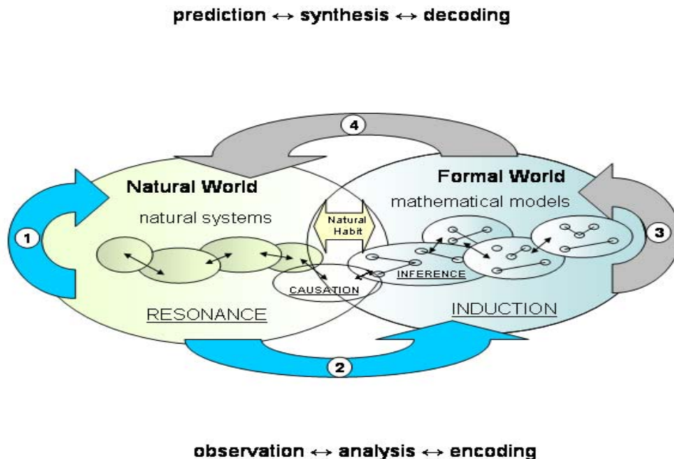
Figure 5: The converging model relation for science
