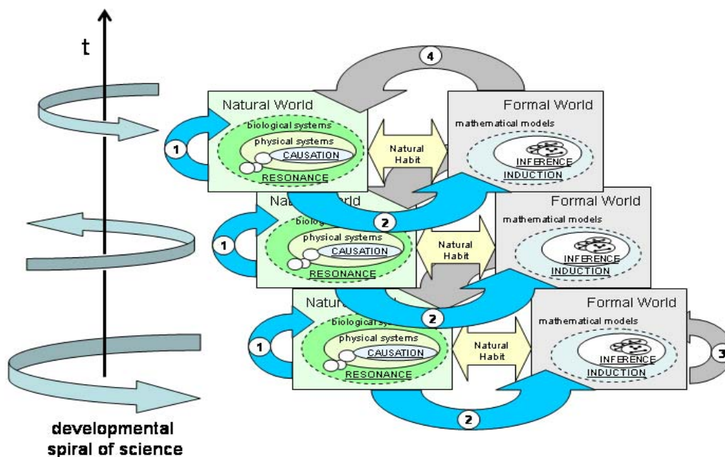
Figure 4: The evolving modelling relation for science
